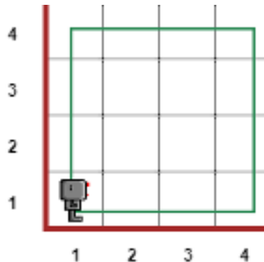
(a) Reeborg_pattern2
