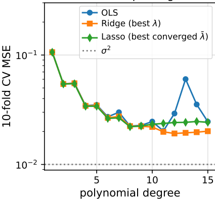
best model per degree
