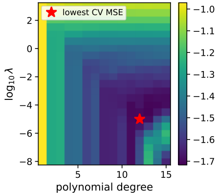
Ridge: \log_{10} CV MSE
