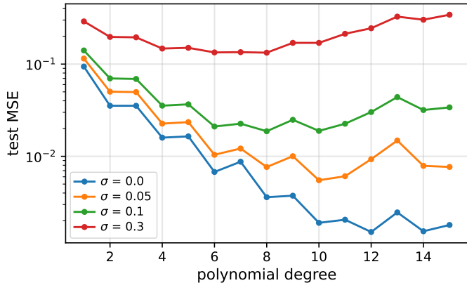
varying \sigma ( n = 100 )
