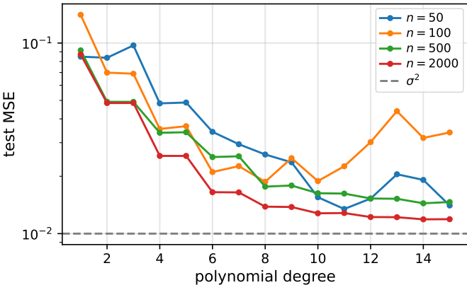
varying n ( \sigma = 0.1 )
