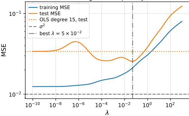
MSE against the penalty
