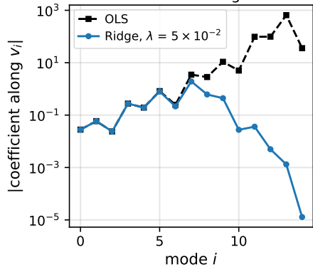
coefficients in the singular basis
