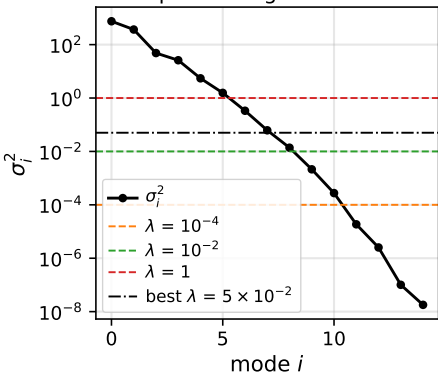
squared singular values
