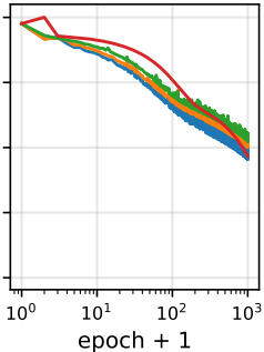
AdaGrad, \eta = 0.1
