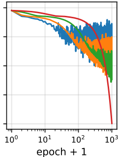
Adam, \eta = 0.005
