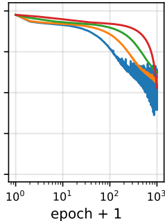
RMSprop, \eta = 0.001
