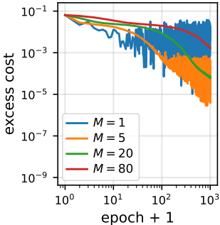
plain, \eta = 0.02
