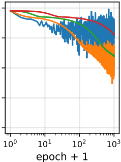
momentum, \eta = 0.002
