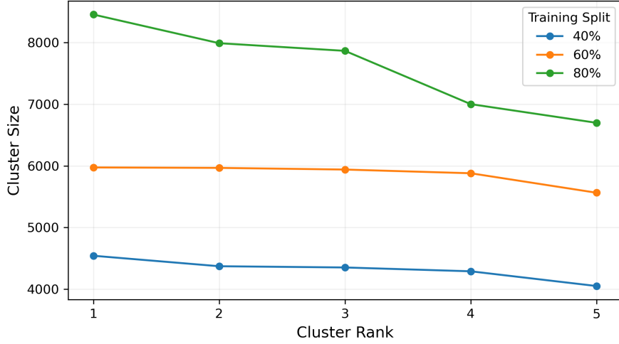
Figure 5: Sizes of the five largest user clusters for each training split, using ALS setting 2 user factors and k -means clustering with k = 25 .
