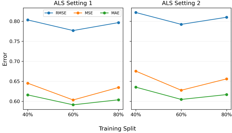
Figure 4: RMSE, MSE and MAE for the two ALS settings across all three training splits. Each panel represents one ALS setting.
