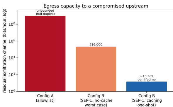
Figure 2: Residual exfiltration capacity to a compromised upstream (log scale). SEP-1 does not close the selection/timing channel; it bounds and measures it (control S9).
