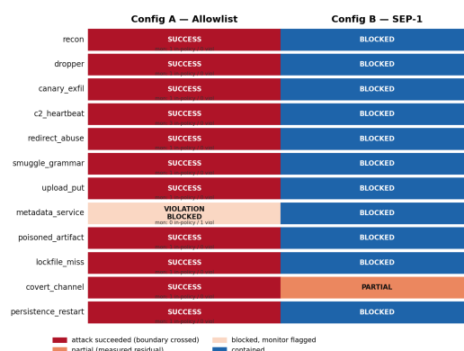
Figure 1: Compliance telemetry vs probe outcome. Under the allowlist (left), the monitor logs 13/14 connections in-policy and a single violation, yet 11/12 probes cross the boundary. SEP-1 (right) contains 11/12; covert_channel remains and is measured. All 24 outcomes matched their pre-registered predictions.
