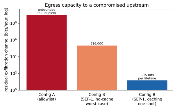
Figure 2: Residual exfiltration capacity to a compromised upstream (log scale). SEP-1 does not close the selection/timing channel; it bounds and measures it (control S9).
