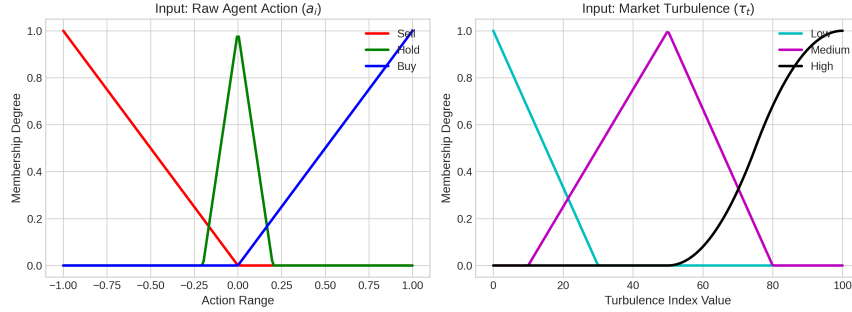
Figure 7: Membership functions for the Fuzzy Action Smoother, mapping the partitions for the raw agent action input a_i (left) and the current market turbulence index \tau_t (right).
