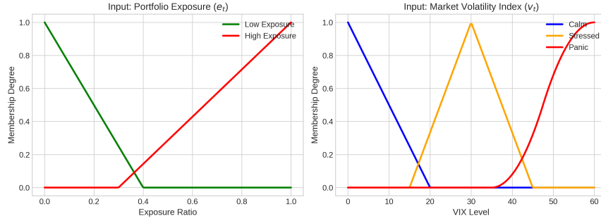
Figure 8: Membership functions for the Fuzzy Reward Shaper, showing the continuous state intervals defined for portfolio exposure e_t (left) and the VIX volatility metric v_t (right).
