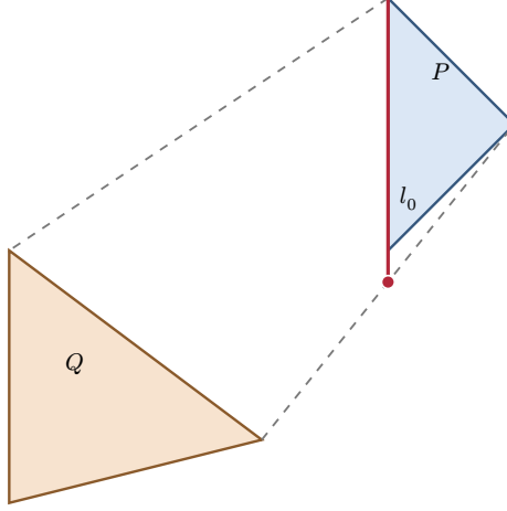
Figure 1: The separator l_0 is the extension of the first geodesic segment; it terminates on a bridge and does not intersect Q , so the cut q_0^+ does not exist.
