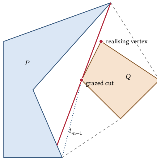
Figure 2: The last separator is anchored on P at both ends and passes through a vertex of Q without terminating into Q 's wall; the realising vertex lies beyond the grazed cut, which shields nothing.
