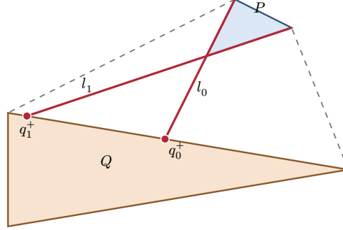
Figure 3: l_1 's backward extension lands before l_0 's cut in boundary order ( q_1^+ precedes q_0^+ ), so the fixed-direction subchain scan between the cuts wraps around Q .
