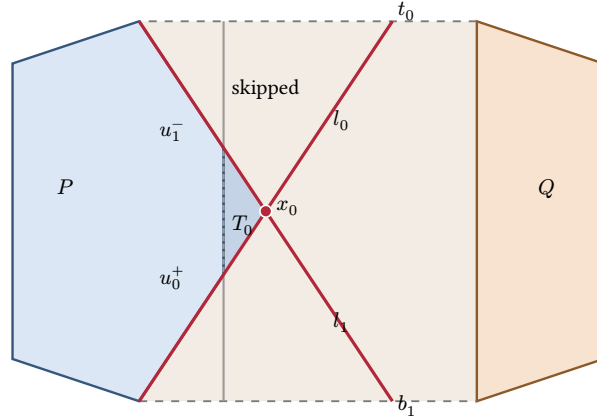
Figure A.2: A skip. The geodesic turns left twice on P' ; the extension of its first segment ( l_0 ) meets the extension of its third ( l_1 in the kept sequence) at x_0 , so Step 1(d) skips the middle segment's extension (grey). The skipped chain is the single P' edge from u_0^+ to u_1^- , and the region T_0 (dark) it bounds with the two arm pieces is a convex triangle. Both kept separators land on bridges, so every subchain but P_1 runs to a sentinel; P_1 starts at p_0^+ = u_0^+ .
