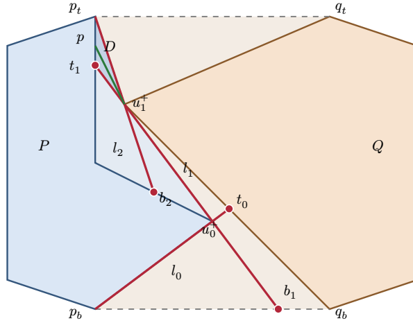
Figure A.1: Pockets and arms. The geodesic (dotted) turns left at the P' vertex u_0^+ = (4, 3) and right at the Q' vertex u_1^+ = (1, 7) , cutting the channel into a P -pocket (blue) and two Q -pockets (sand). The two arms at u_0^+ enter the bottom Q -pocket and land on Q' ( t_0 ) and on the bottom bridge ( b_1 ); the two arms at u_1^+ enter the P -pocket and land on P' ( t_1, b_2 ). The upper arm of l_1 cuts the region D (dark) off the P -pocket. The green sight from p = (0, 9) to q = u_1^+ touches l_1 only at q : it lies above the cut t_1 of subproblem 1 and is covered by subproblem 2, whose subchains both run to their sentinels.
