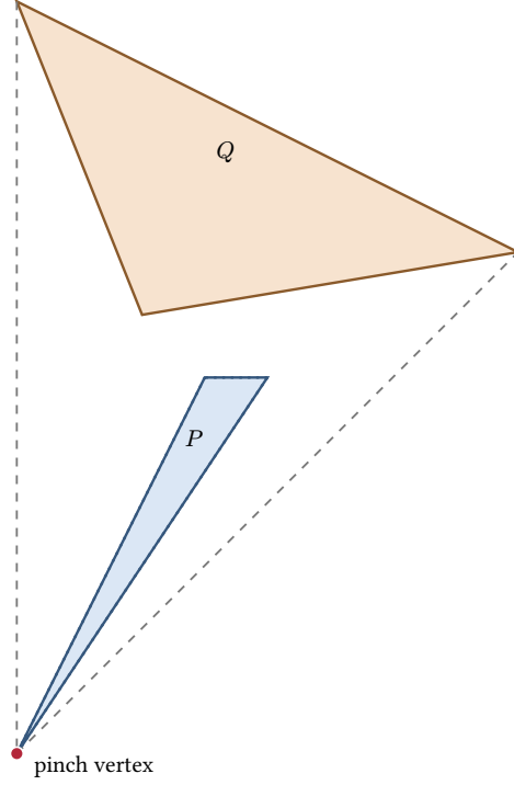
Figure 4: Both supporting segments (dashed) share P 's single hull contact: the channel is pinched there, and the shortest path (dotted) wraps around P between the two instances of the pinch vertex.
