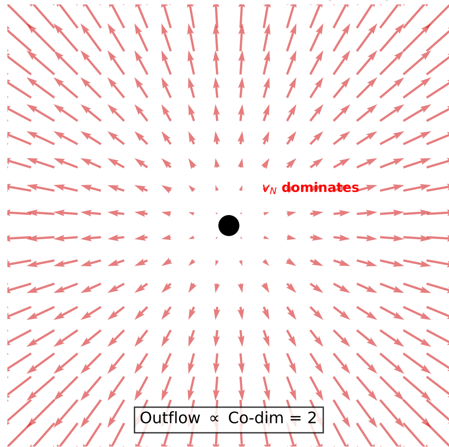
(b) Low LID ( d = 0 ): Point Singularity
