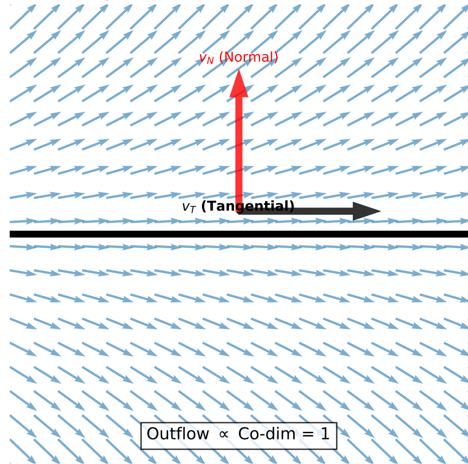
(a) High LID ( d = 1 ): Preserved Manifold
