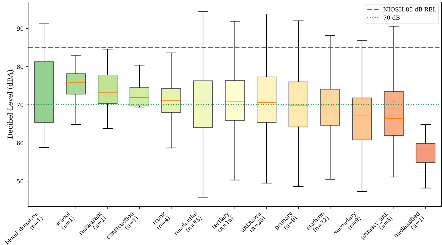
GoPro Noise Readings by Road Type
