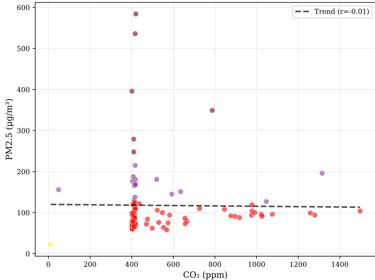
PM2.5 vs CO 2 Correlation (N=98)
