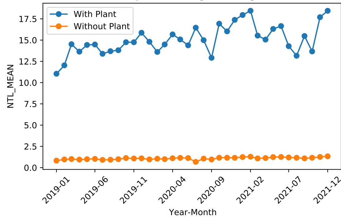
Comparison of Nighttime Lights
