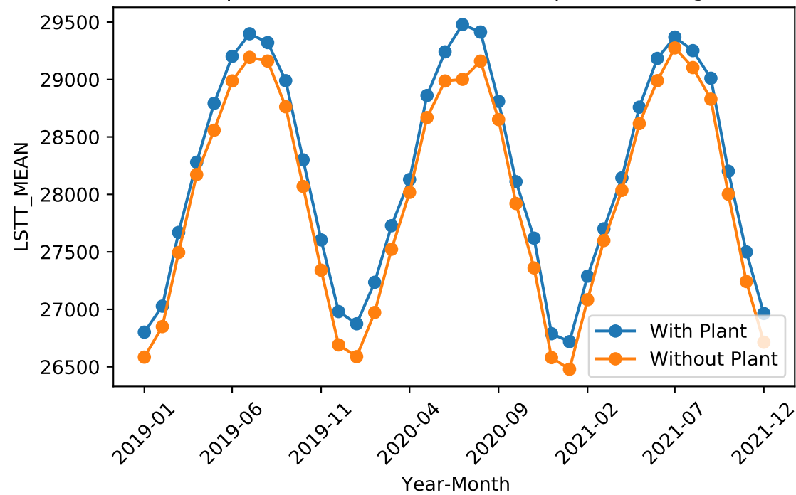
Comparison of Land Surface Temperature (Night)
