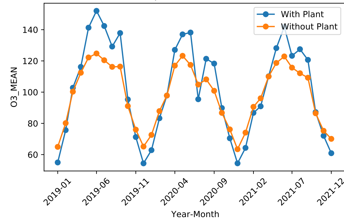
Comparison of O3 Means
