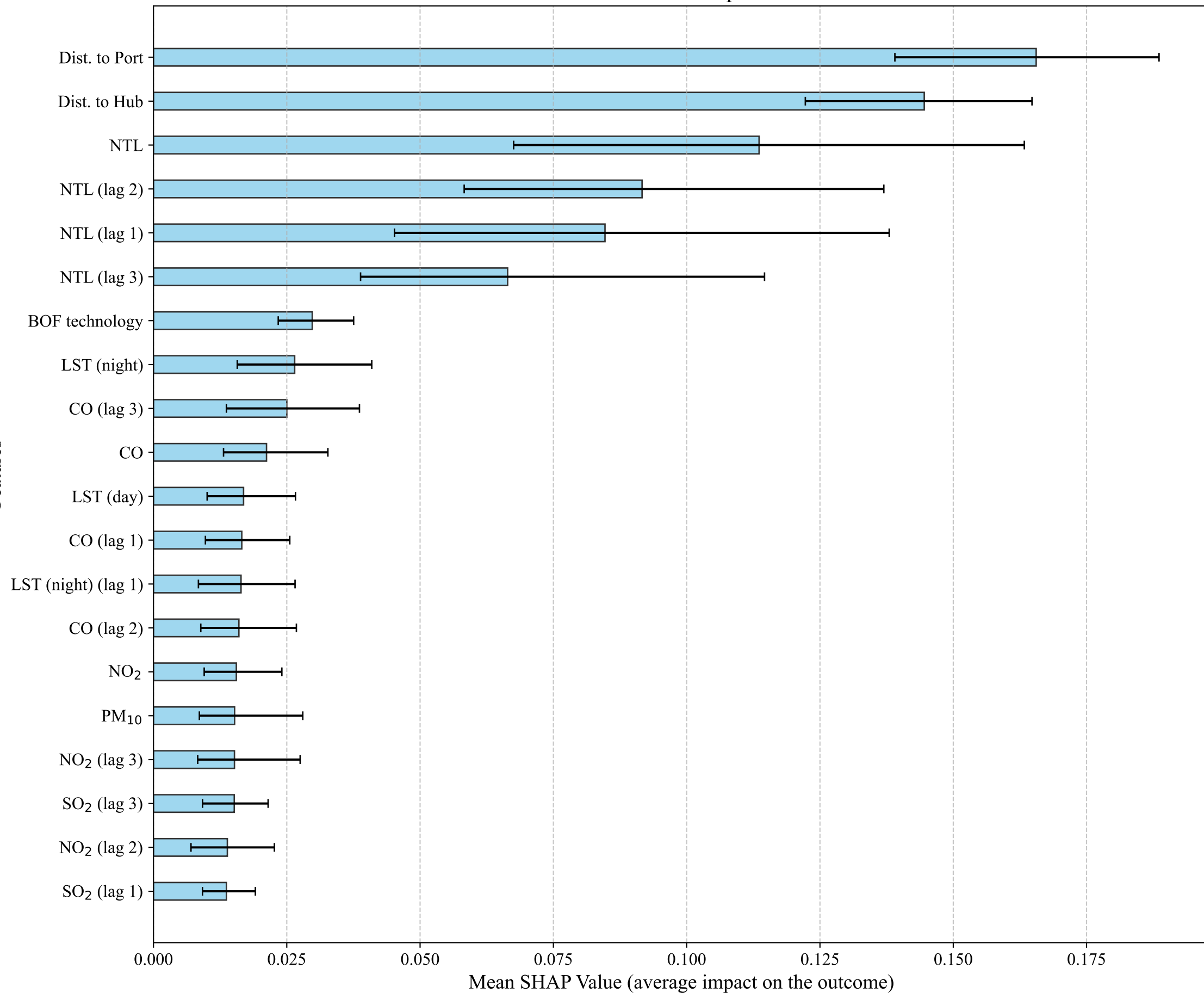
Global Feature Importance
