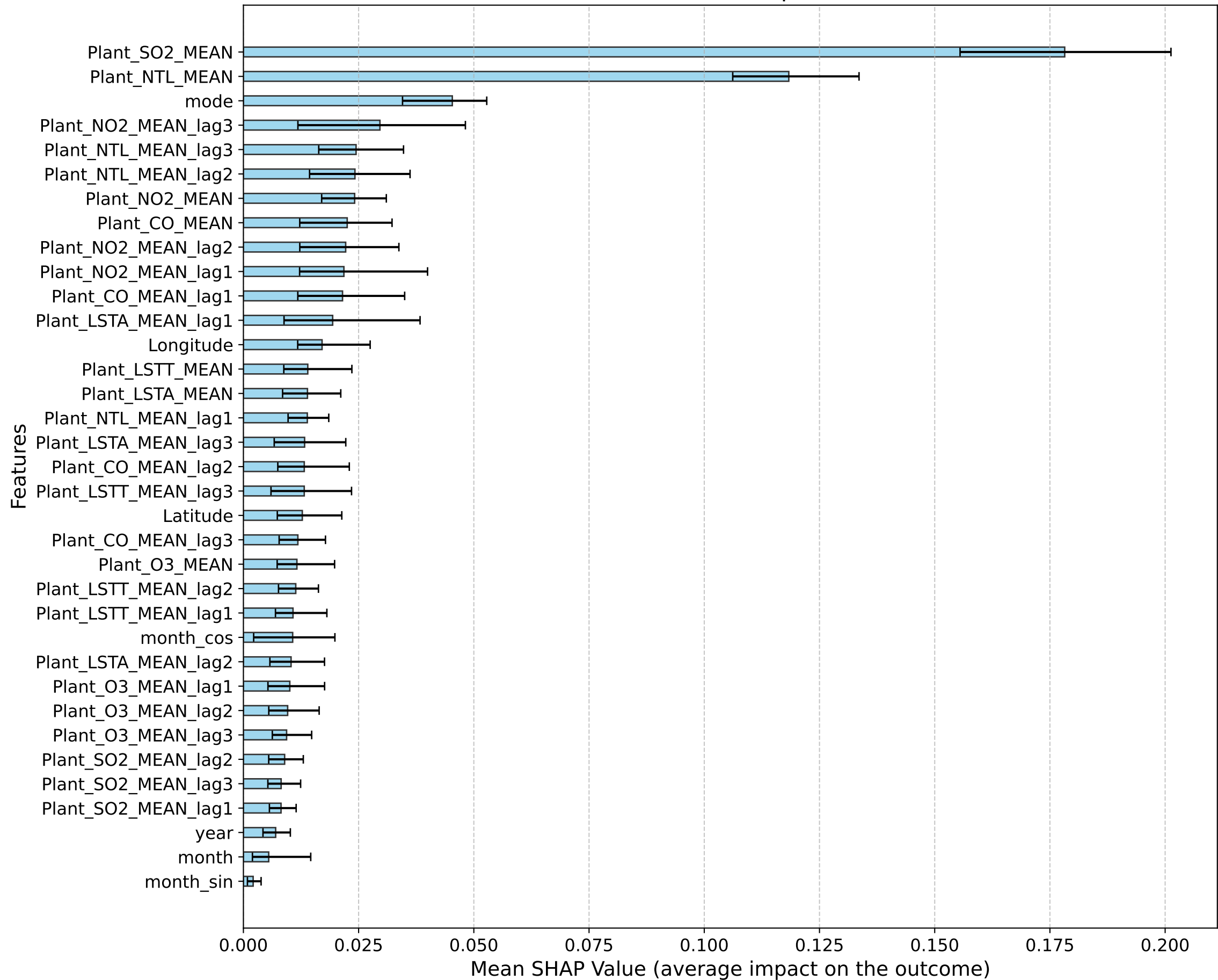
Global Feature Importance
