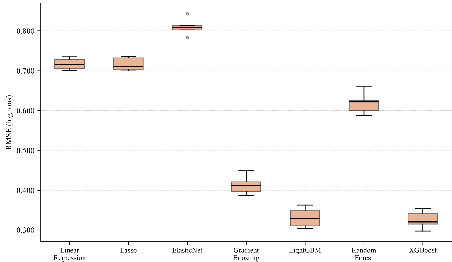
Plant-Level Output Model: RMSE (5-Fold CV)
