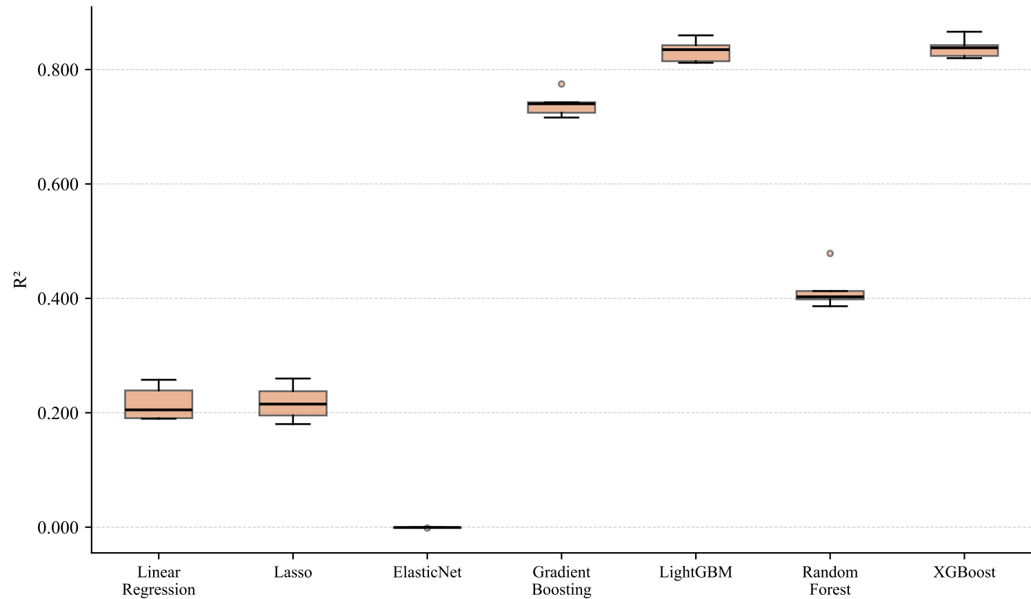
Plant-Level Output Model: R^2 (5-Fold CV)
