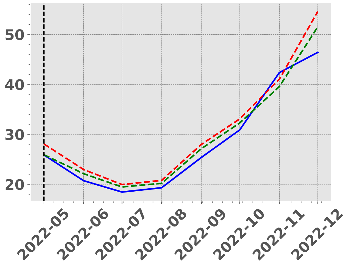
PM2.5
