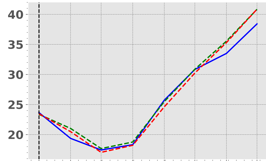
PM10
