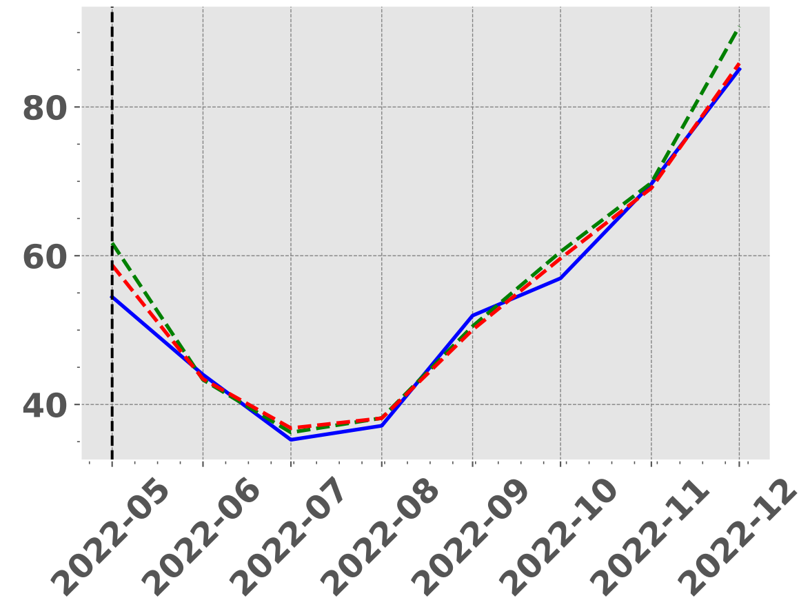
PM10
