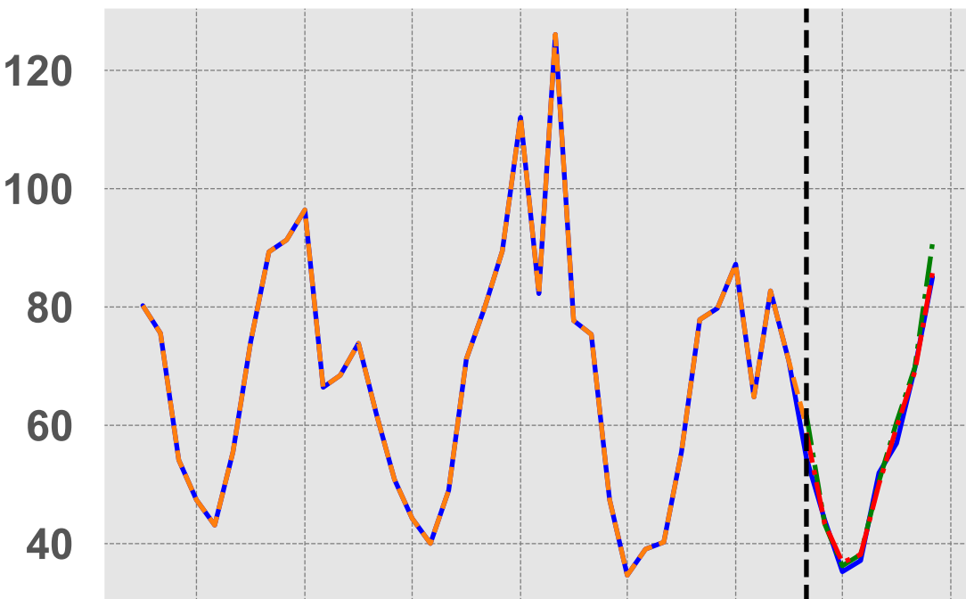
PM10
