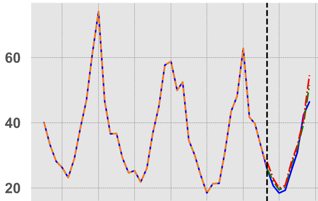
PM2.5
