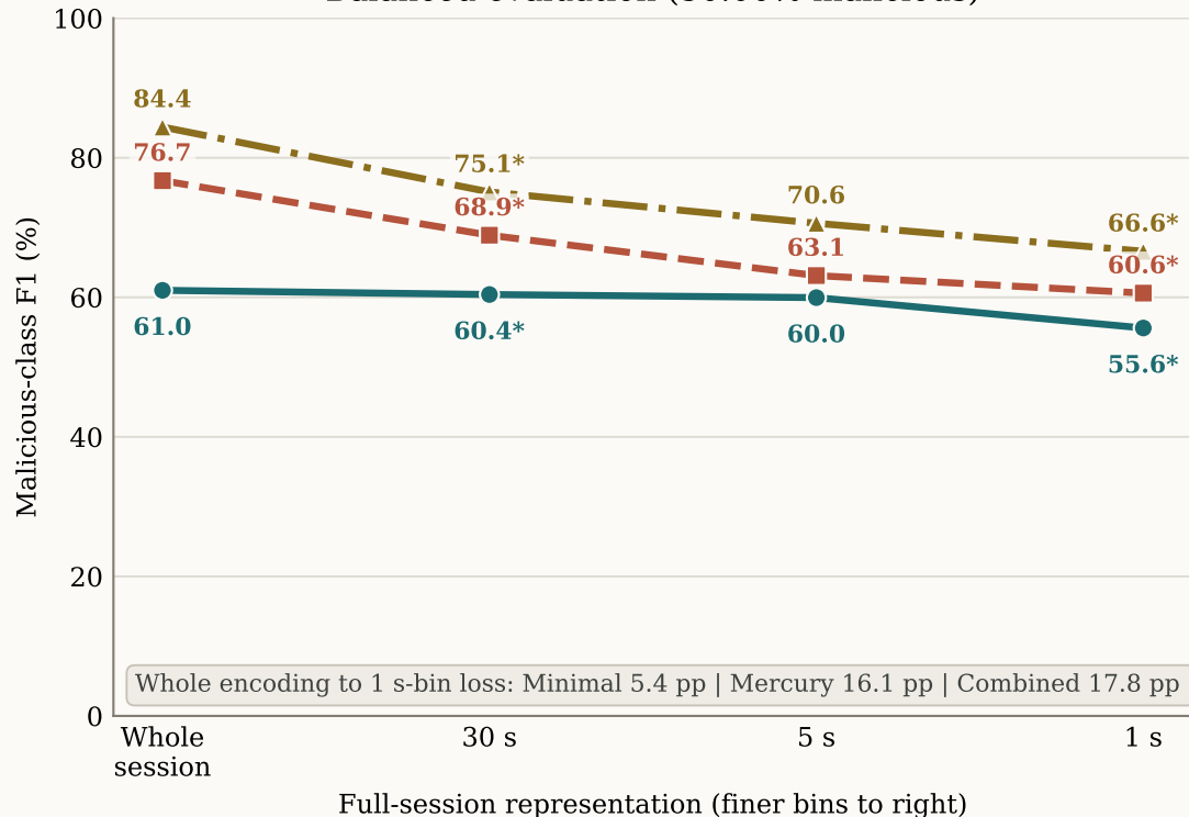
Balanced evaluation (50.00% malicious)
