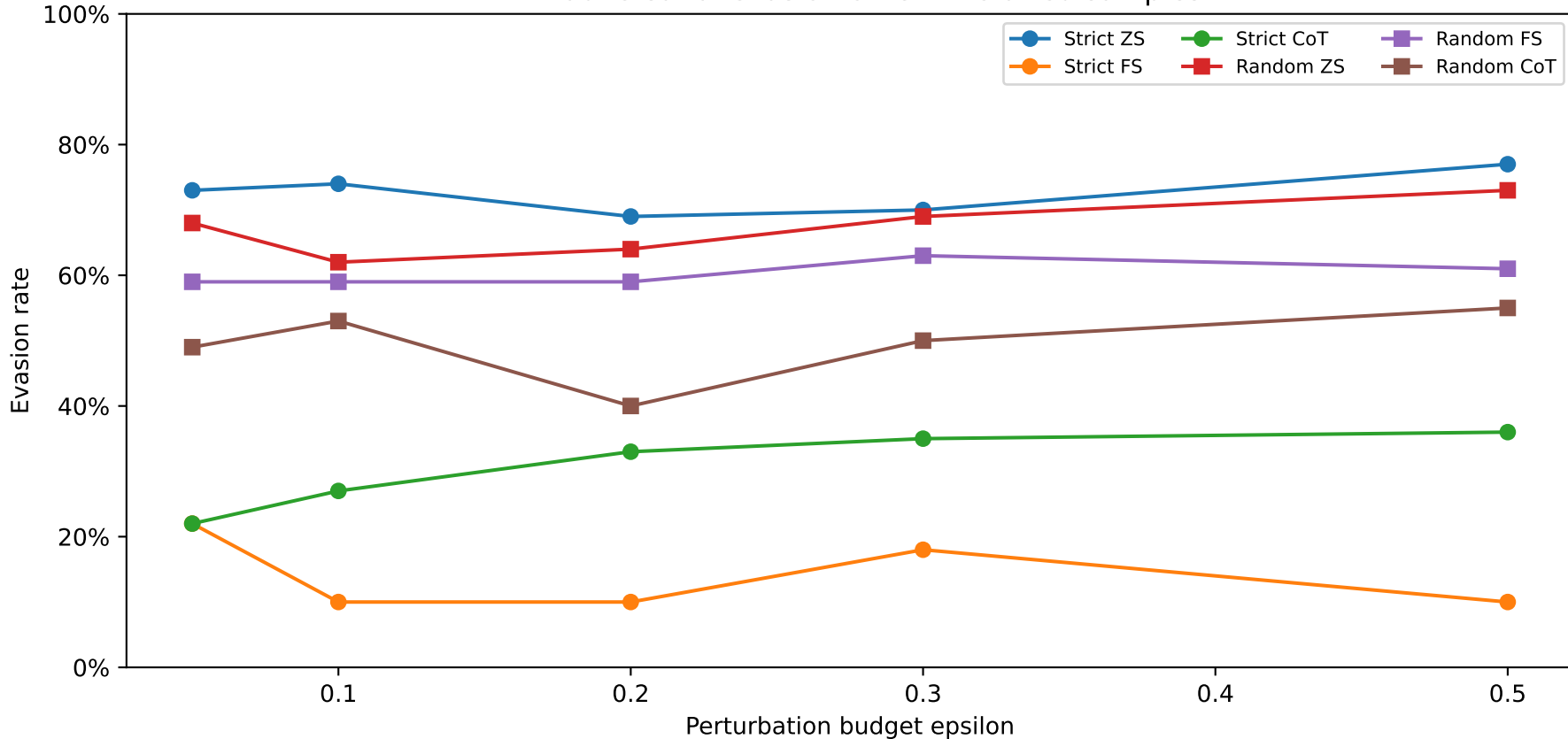
LLM adversarial evasion on CART-crafted samples
