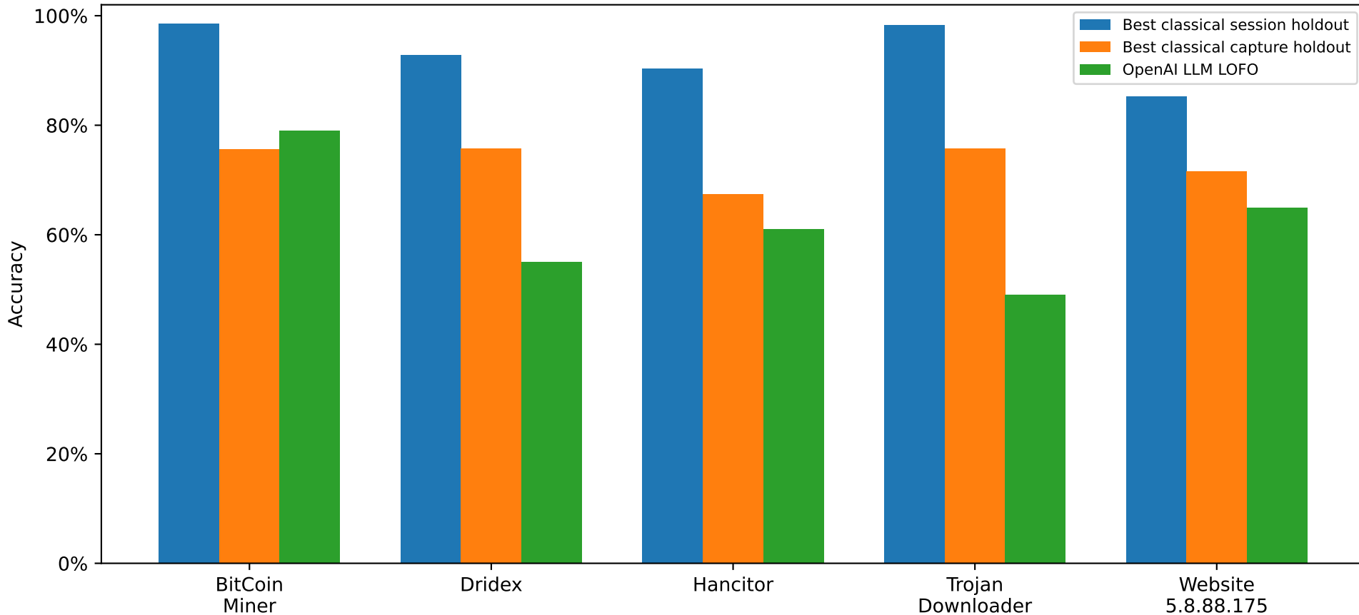
Strict-cluster LOFO accuracy by held-out malware family
