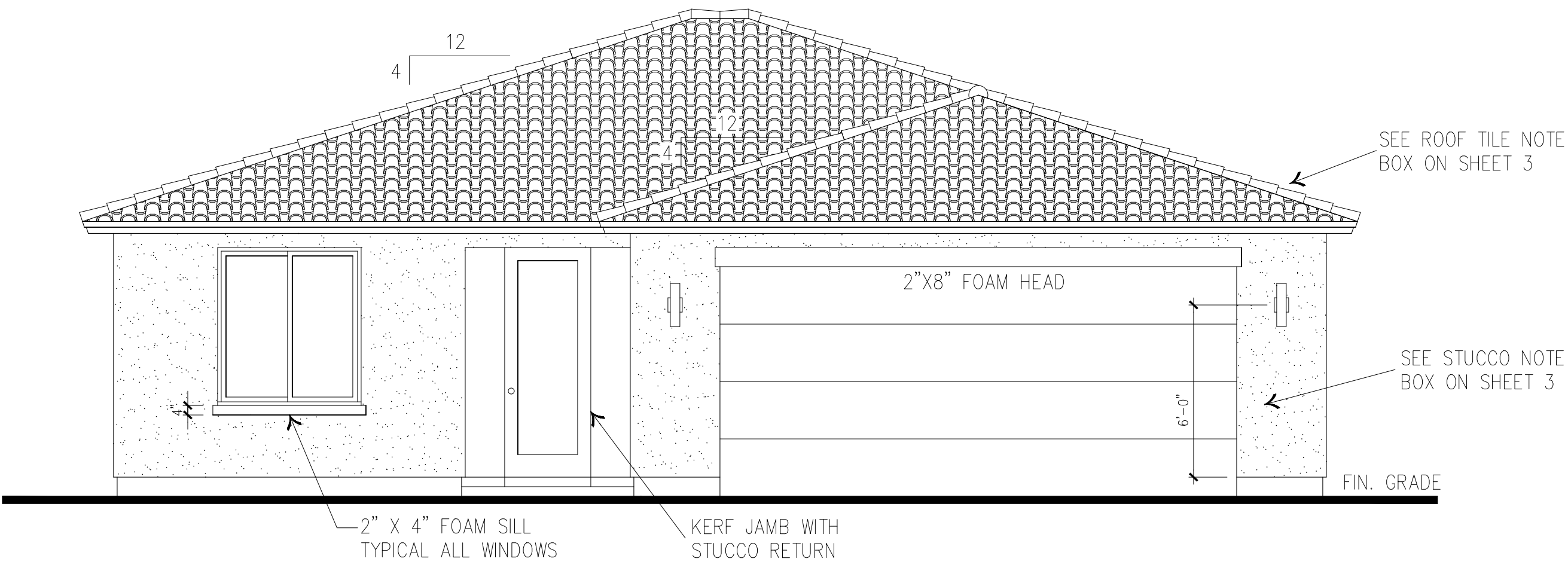
FRONT ELEVATION "C"
