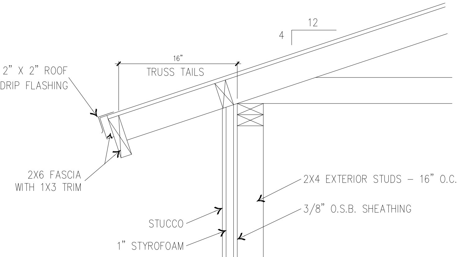
SOFFIT/FASCIA DETAIL
