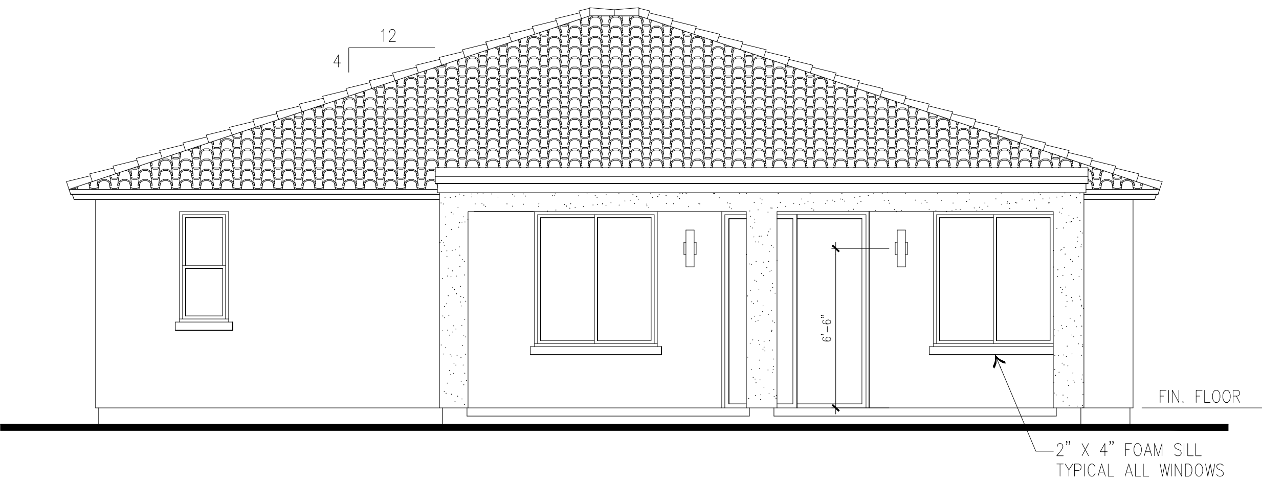
REAR ELEVATION "C"
