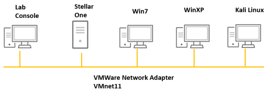
Figure 1 Lab network architecture
