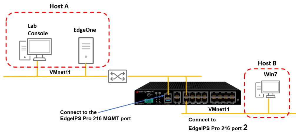
Figure 1 Lab network architecture
