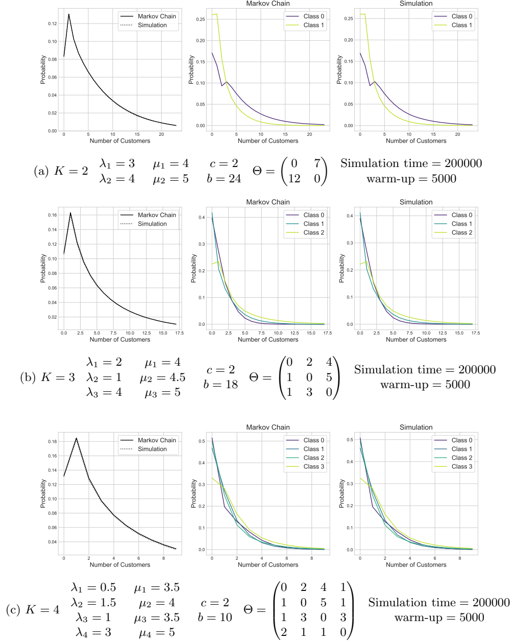
Figure 20: Simulation and Markov chain methods for finding state probabilities for 2, 3, and 4 priority classes.
