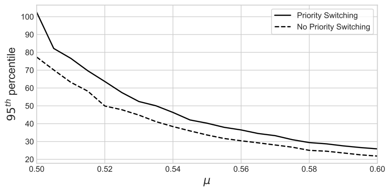
Figure 18: The effect of small increases in the service rate, with and without priority switching.
