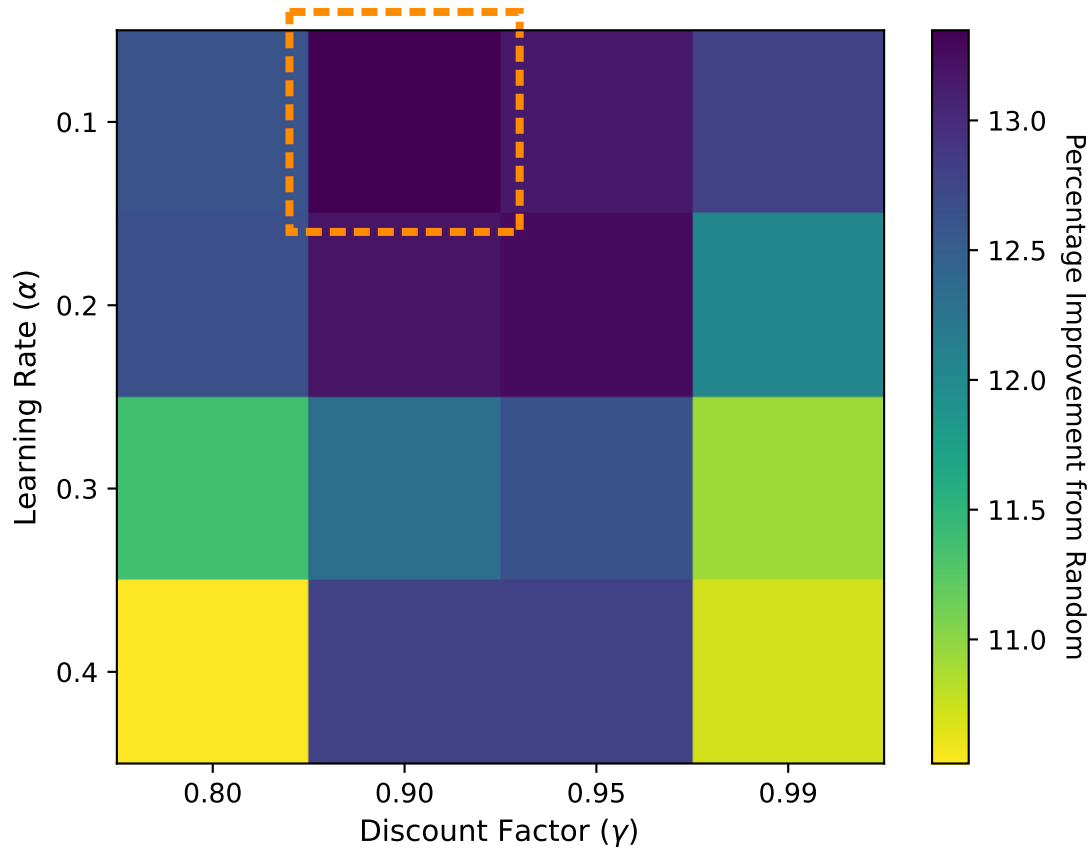
Round 1
