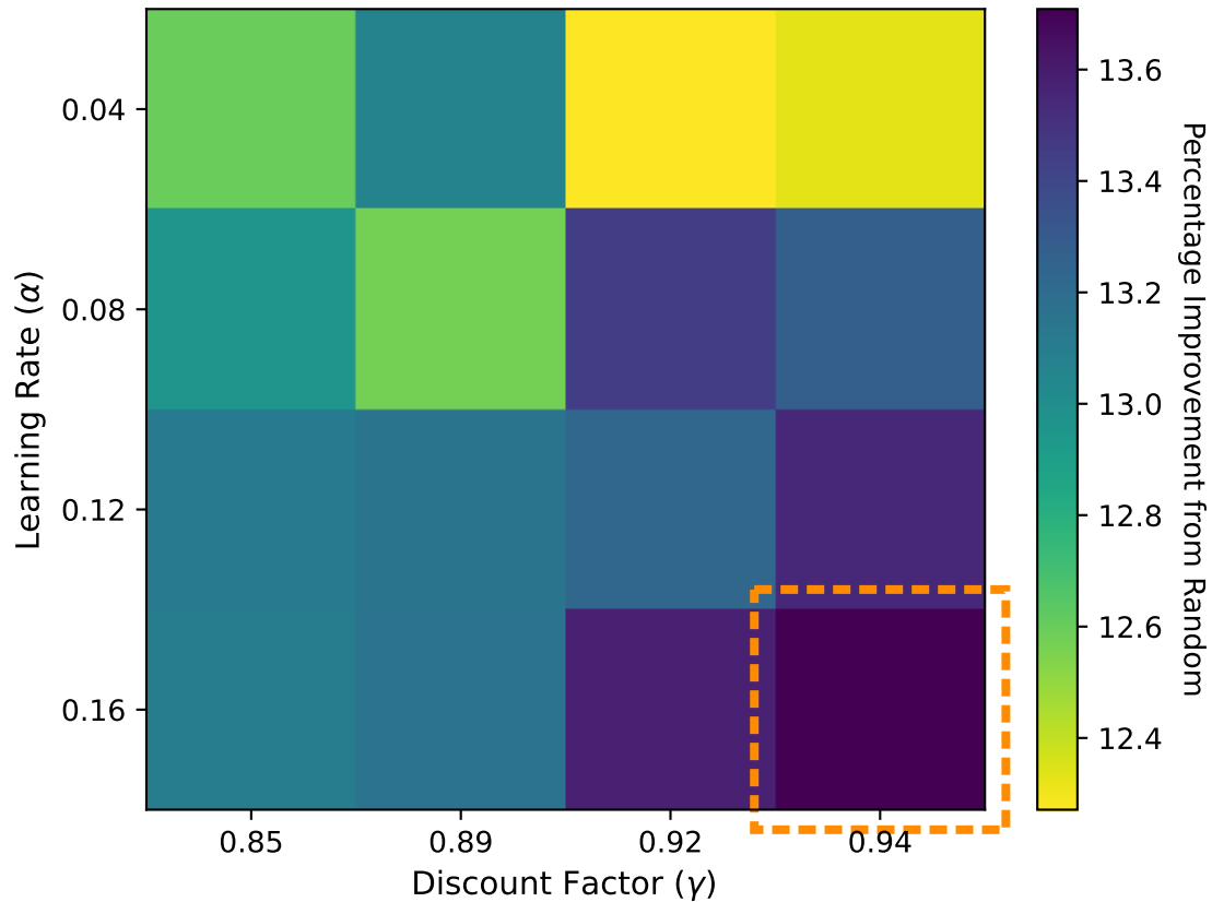
Round 2
