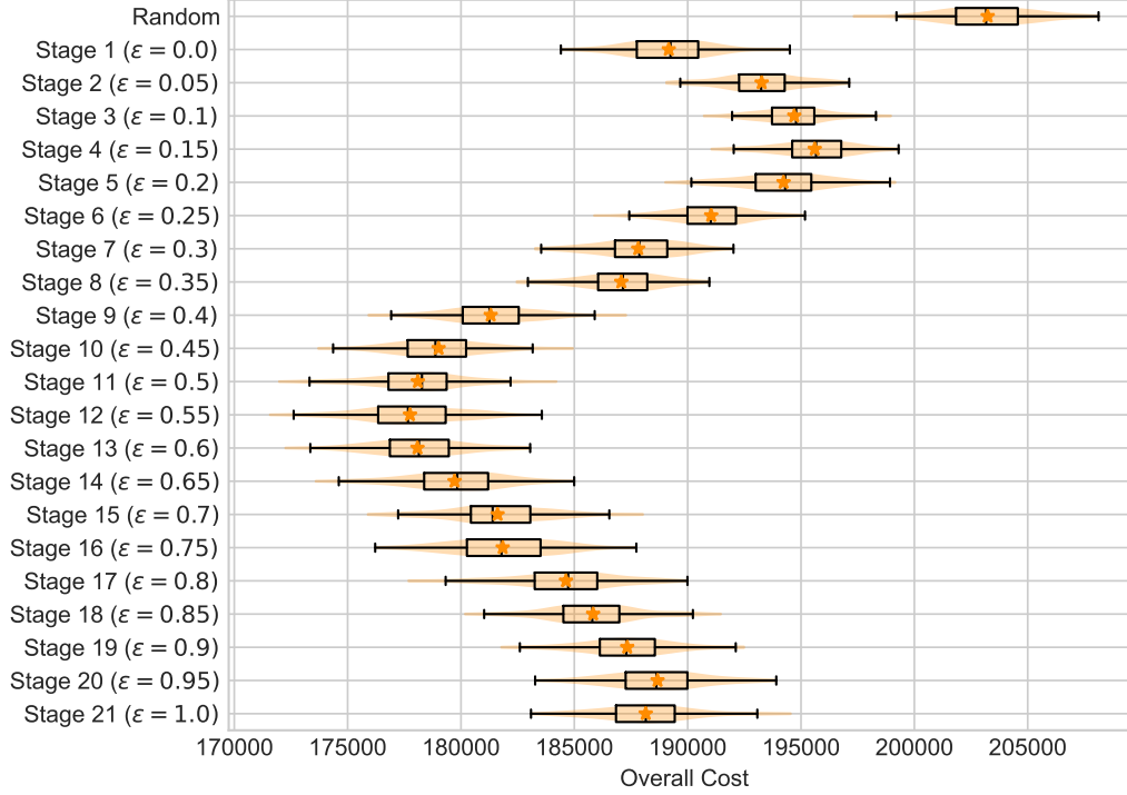
Figure 10: Training curve with tuned hyper-parameters.
