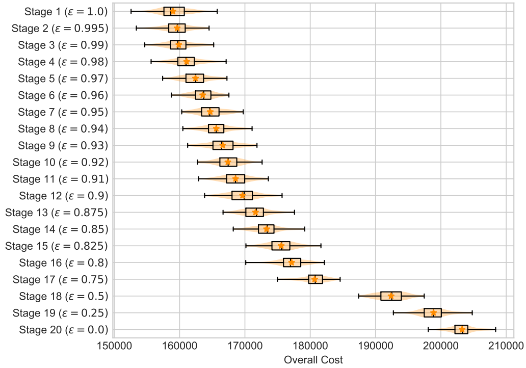
Figure 16: Evaluation of the final best policy (incumbent at Stage 31) when using different exploitation probabilities \epsilon .
