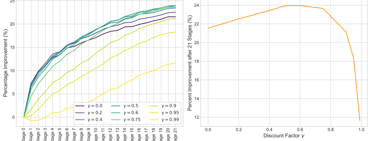
Figure 12: The effect of varying the discount factor \gamma .
