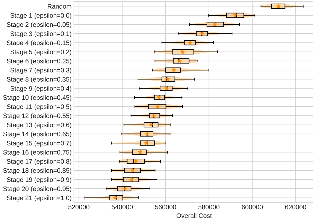
Figure 9: Evaluation of the incumbent policies across the stages.
