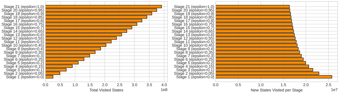
Figure 10: Number of state-action pairs visited in each stage of the training process.
