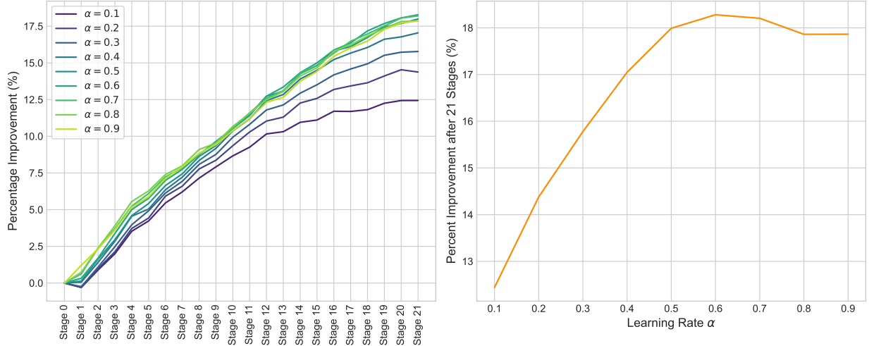
Figure 11: The effect of varying the learning rate \alpha .
