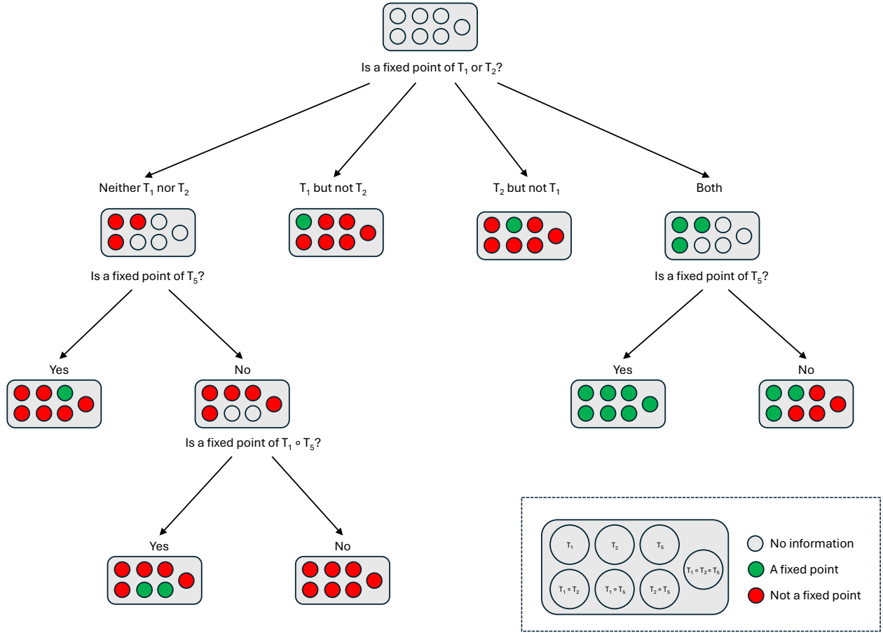
Figure 7: Decision tree to check if a state is a fixed point of a permutation containing T_1 , T_2 , T_5 , or compositions of their combinations.
