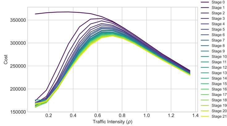
Figure 13: The effect of varying the traffic intensity, \rho .
