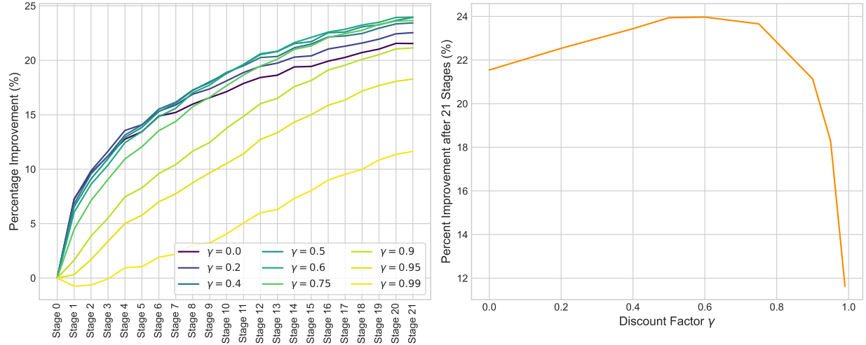
Figure 12: The effect of varying the discount factor \gamma .
