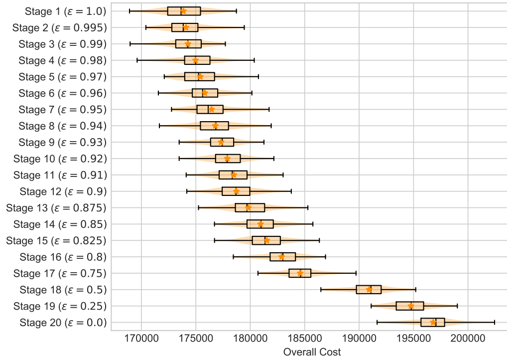
Figure 11: Evaluation of the best policy (incumbent at Stage 15) when using different exploitation probabilities \epsilon .
