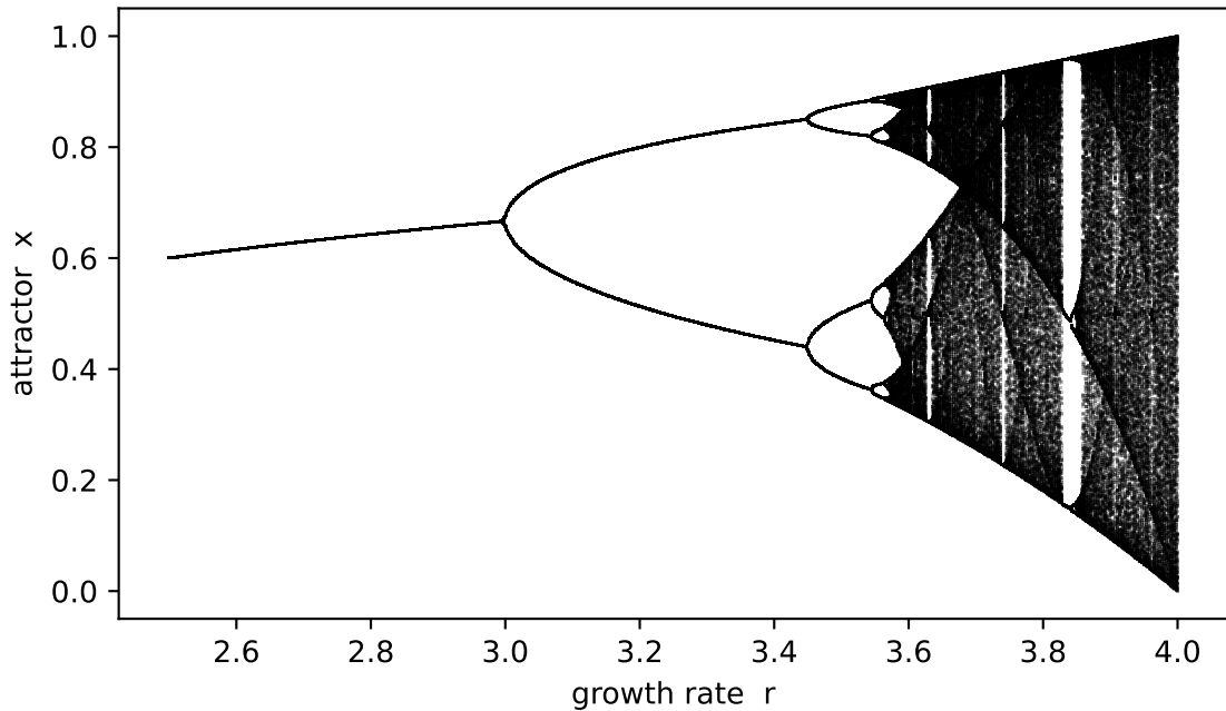
Logistic-map bifurcation diagram
