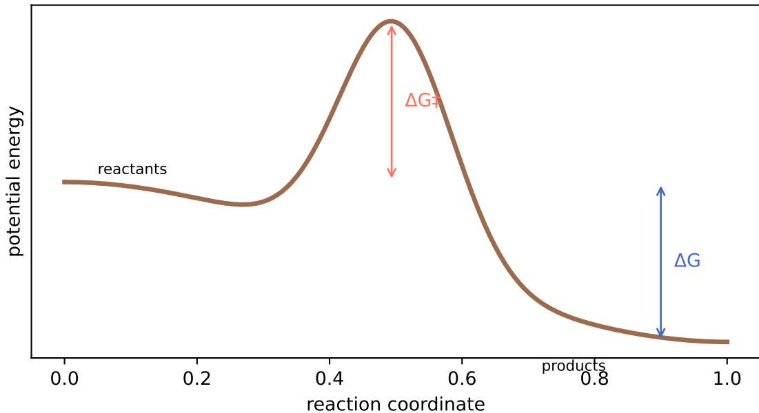
Energy-coordinate diagram
