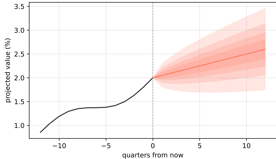
Fan chart — widening ahead
