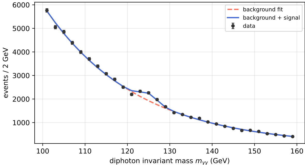
A resonance at 125 GeV
