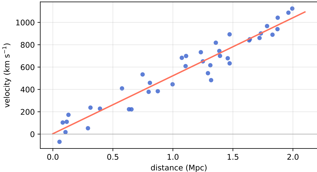
Hubble diagram
