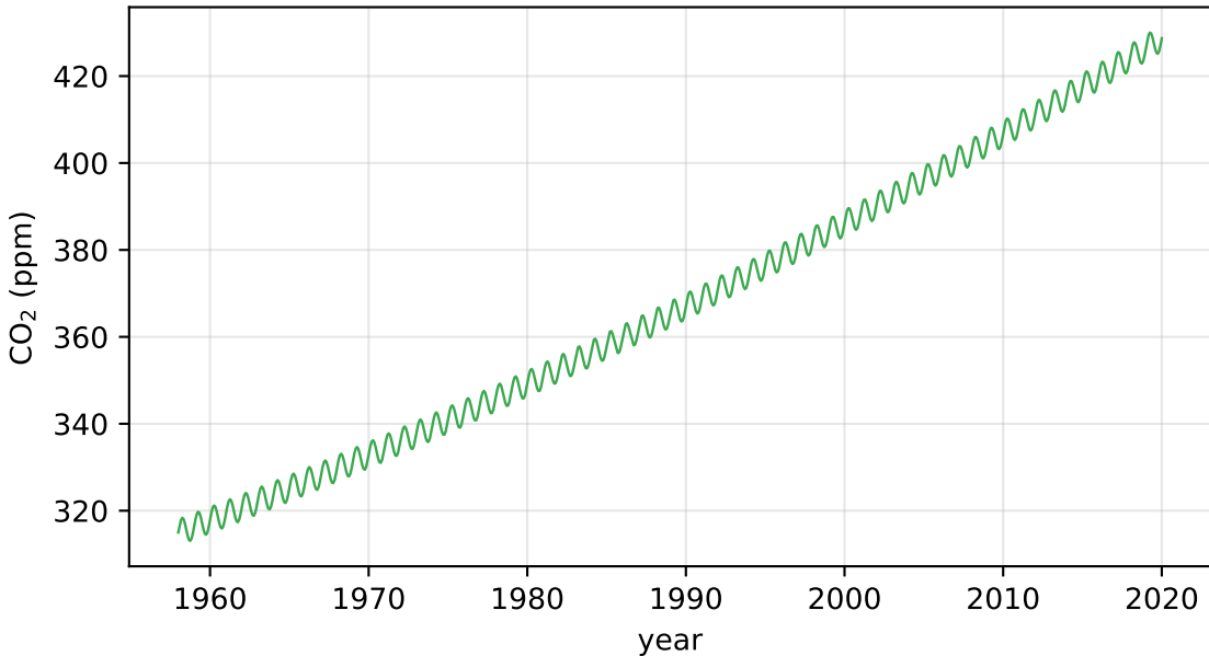
Keeling curve
