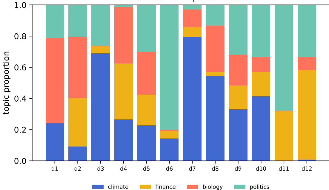
LDA document-topic mixtures
