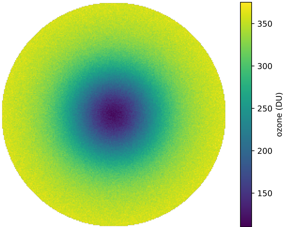
Ozone hole (total column)
