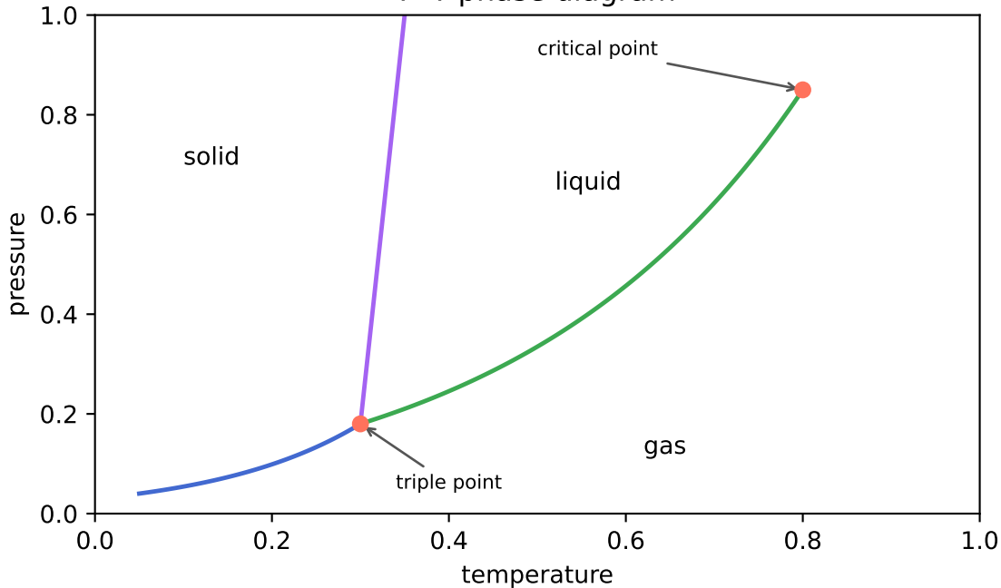
P-T phase diagram
