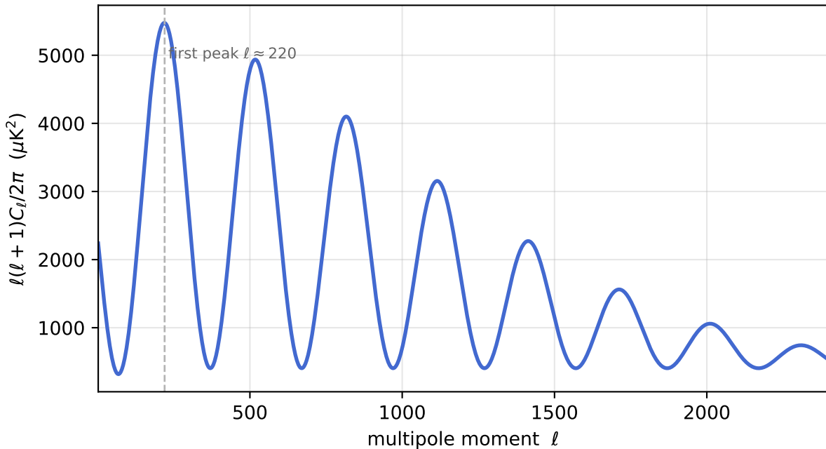
CMB angular power spectrum
