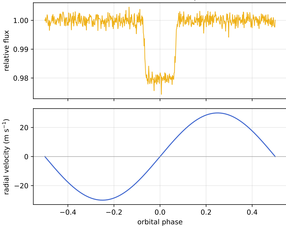
Transit and radial-velocity curves
