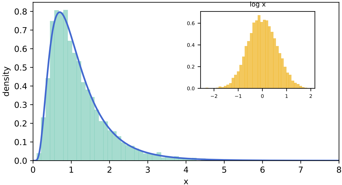
Log-normal distribution
