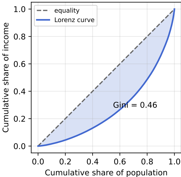
Lorenz curve
