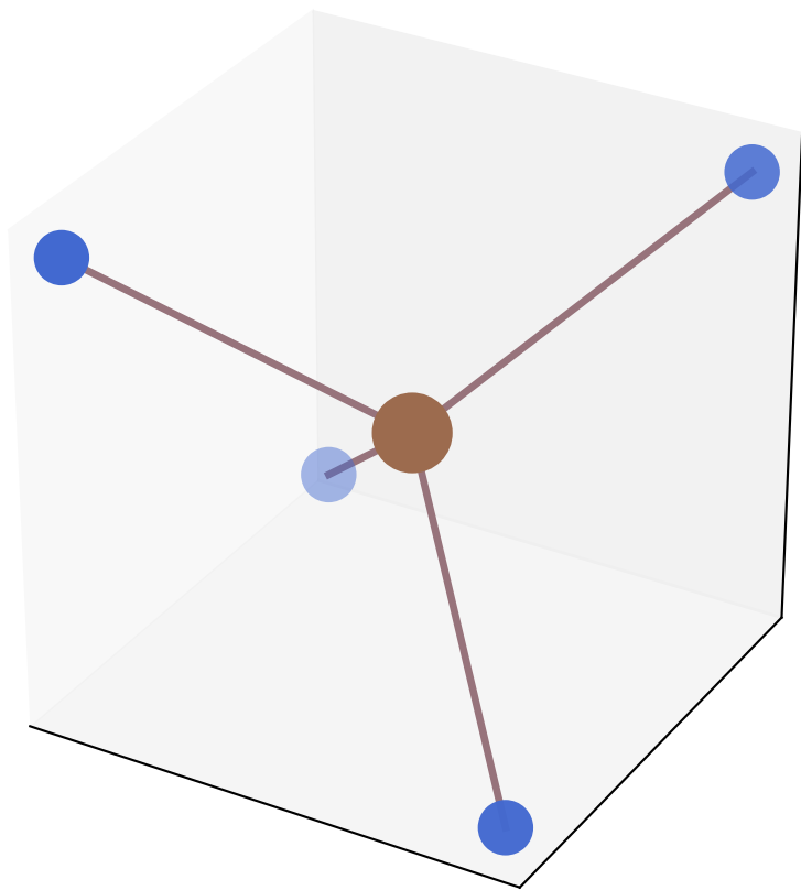
Methane (ball-and-stick)
