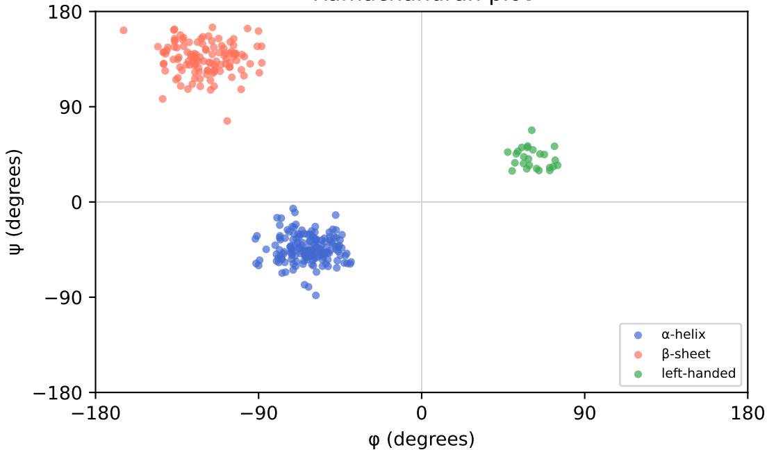
Ramachandran plot
