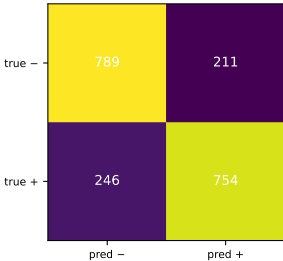
confusion ( \theta = 0.75 )
